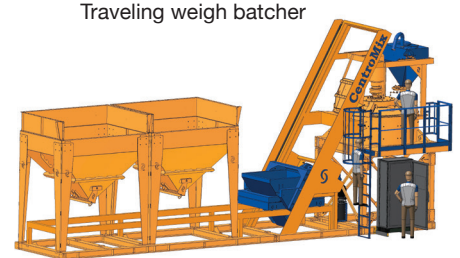
Diagram 4. Traveling weigh batcher
