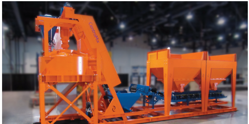
Diagram 3. Aggregate bins with collective belt - exchangeable bins
